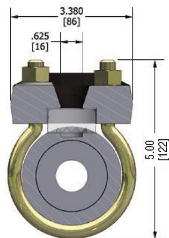
Series RLC Reflex
